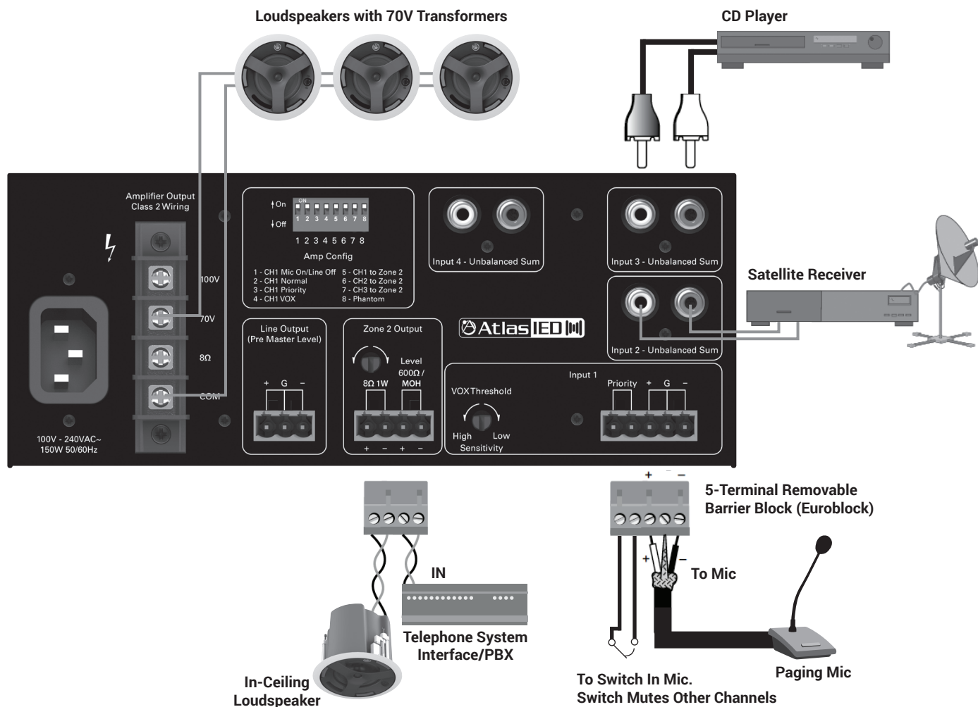
Figure 2.8 Input-Output Wiring
