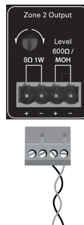
Figure 2.7 Connections to the Telephone (MOH or Amplifier Input) Connector
