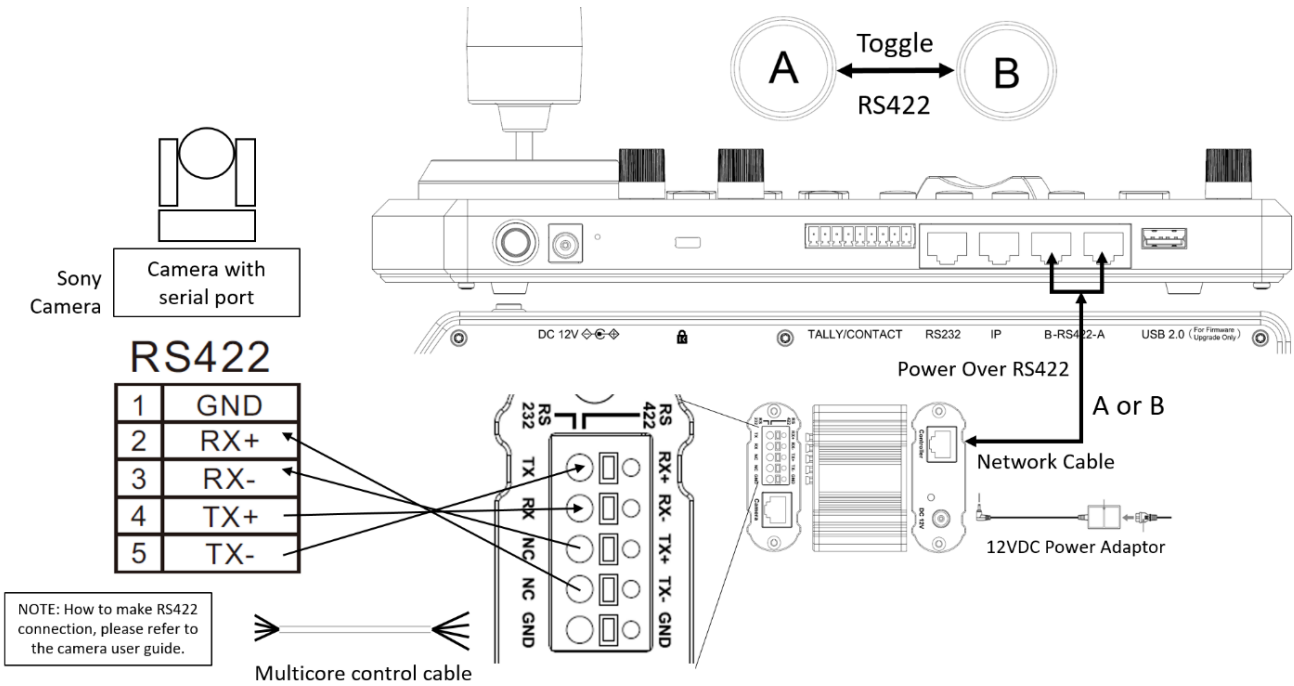
(SONY Camera) RS422 Connection – Via Junction Box - Camera with RS422 serial connector
