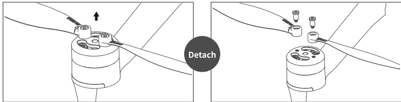
1. Use the screwdriver in the package to press the screw counterclockwise Twist 2 screws out
