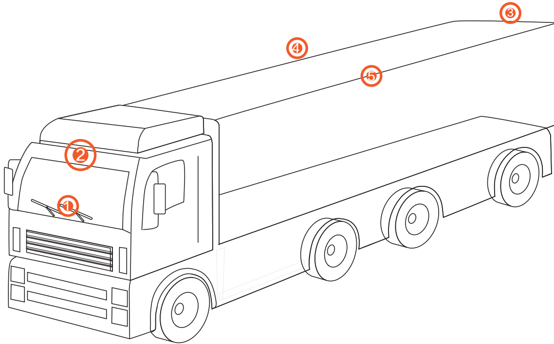
① LCD Monitor ② Front Camera ③ Rear Camera ④ Left Camera ⑤ Right Camera
