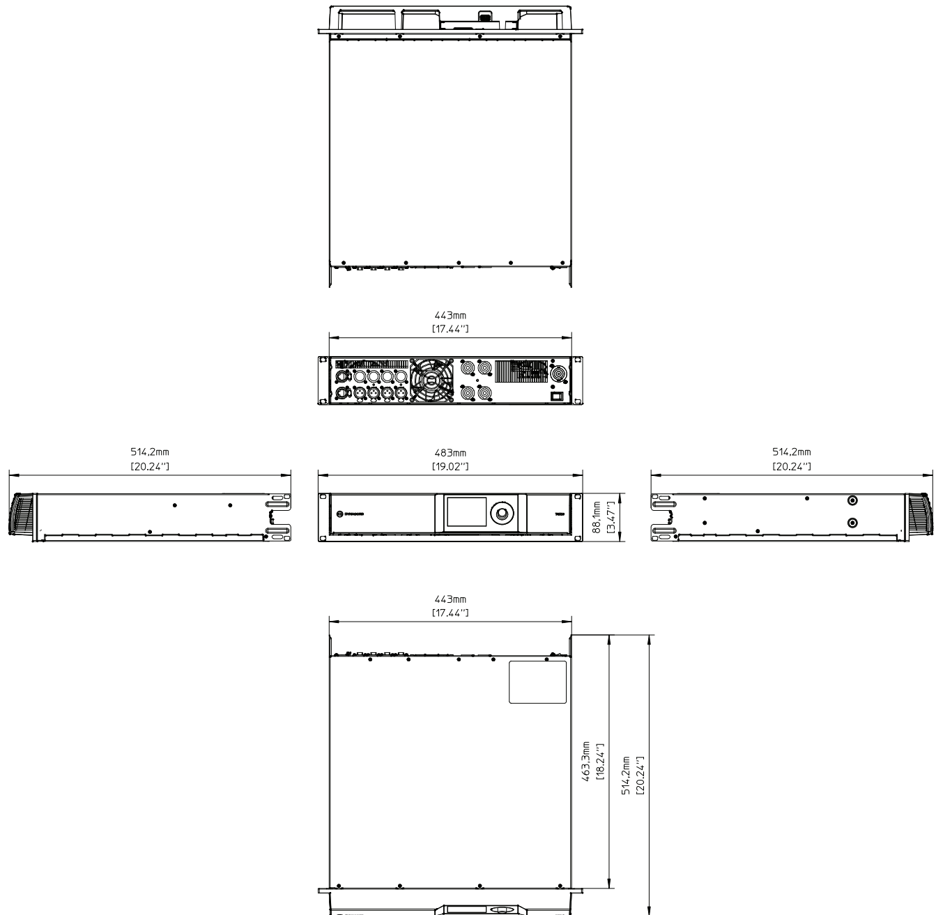
Figure 8.2: Dimensions: TGX
