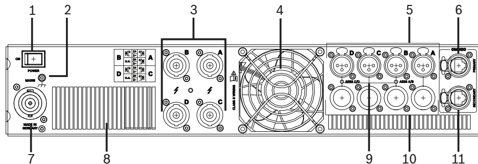
Figure 6.2: TGX rear panel
