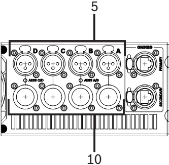
Figure 6.3: TGX audio connectors
