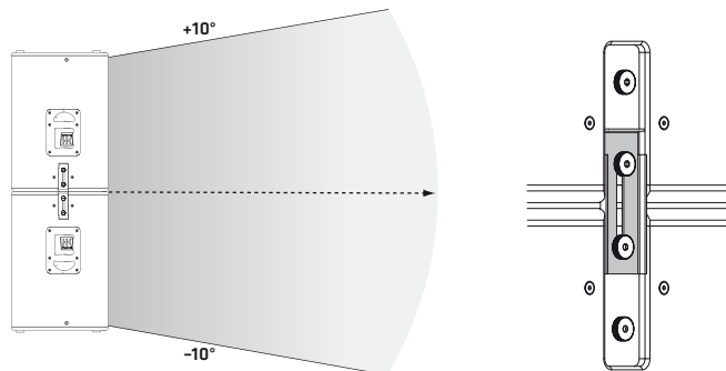
Fig. 5 Headstack
