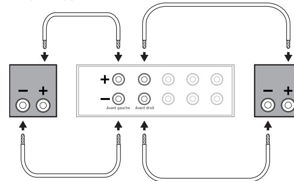
FIGURE 3 BRANCHEMENTS STANDARD
