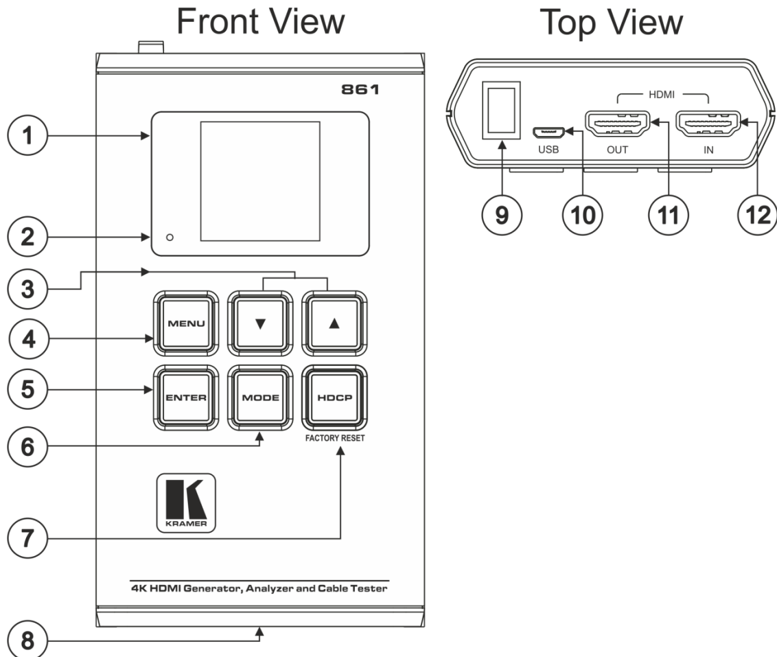
Figure 1: 861 4K HDMI Generator, Analyzer and Cable Tester
