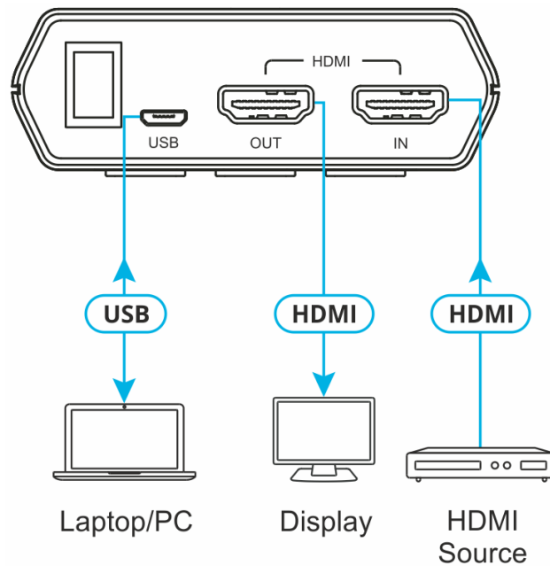
Figure 4: Connection Diagram for Using 232 Commands
