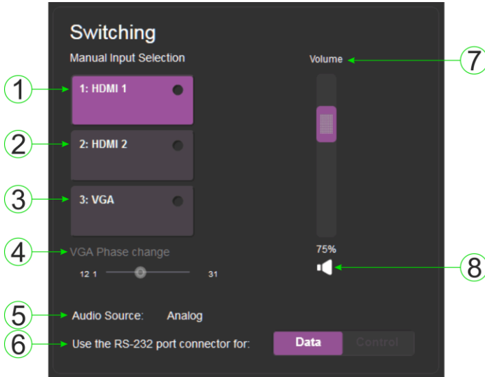
Figure 10: The Switching Page
