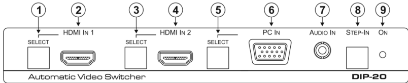
Figure 1: DIP-20 Front Panel
