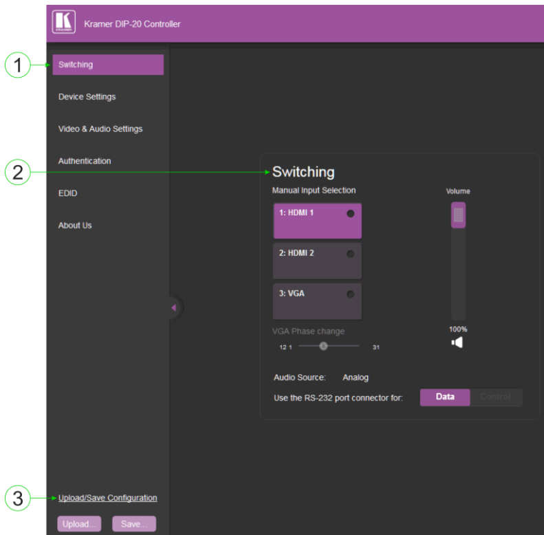
Figure 9: The Main Switching Page
