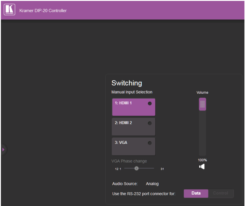
Figure 8: The Default Page
