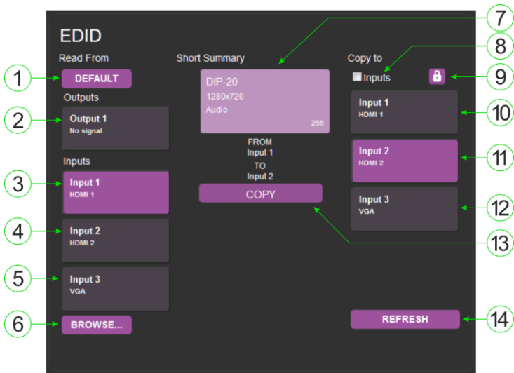
Figure 14: The EDID Page
