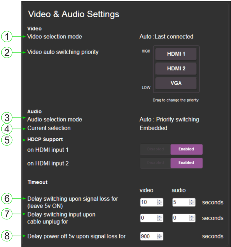
Figure 12: The Video and Audio Settings Page
