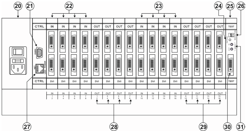
Figure 3: VS-1616D Rear Panel Showing DVI cards
