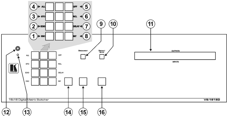
Figure 1: VS-1616D Front Panel
