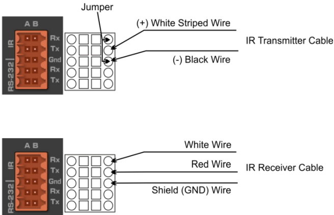
Figure 14: Connecting IR Emitter / Receiver
