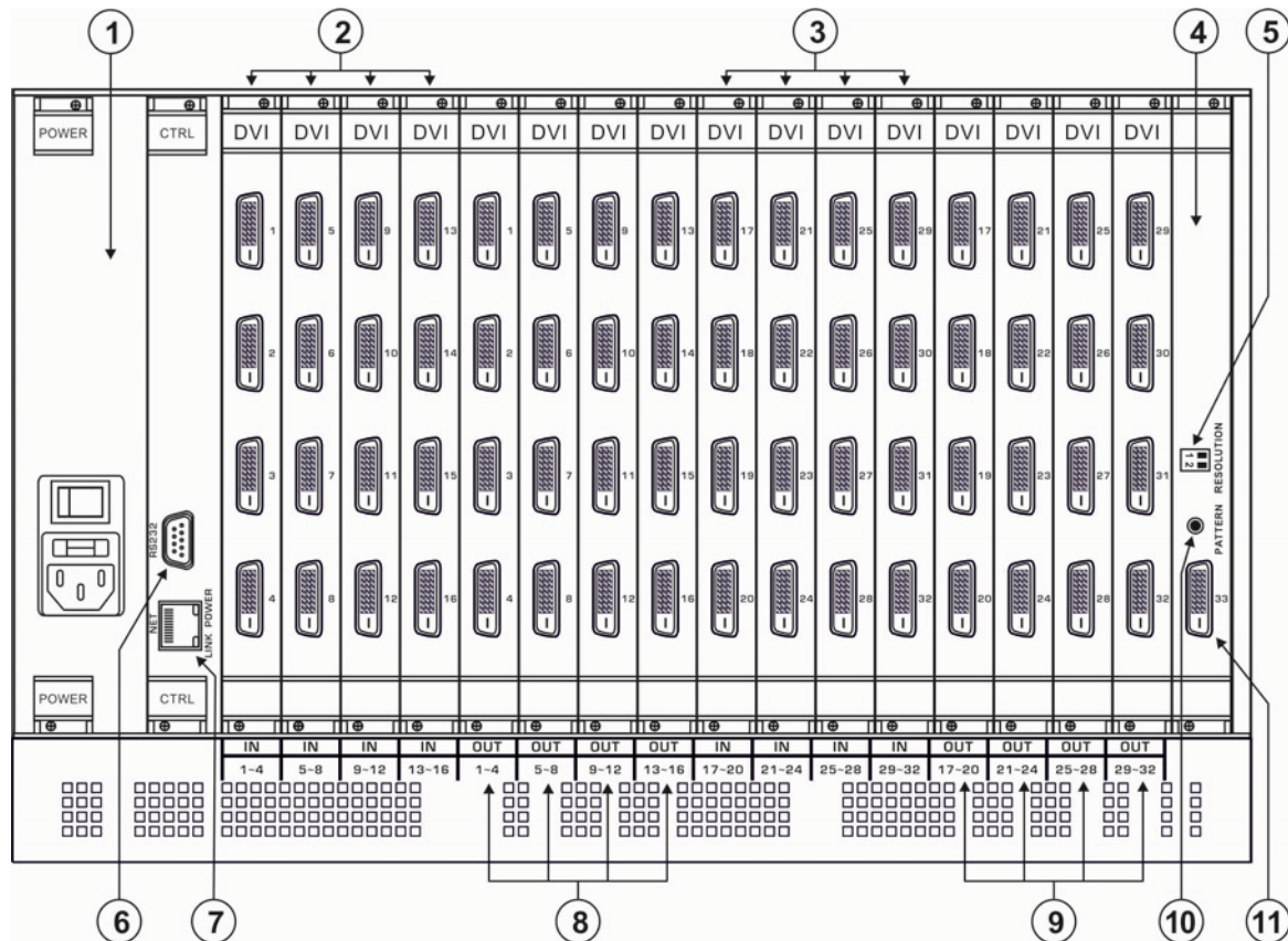
Figure 3: VS-3232DN 32x32 Digital Matrix Switcher Rear Panel
