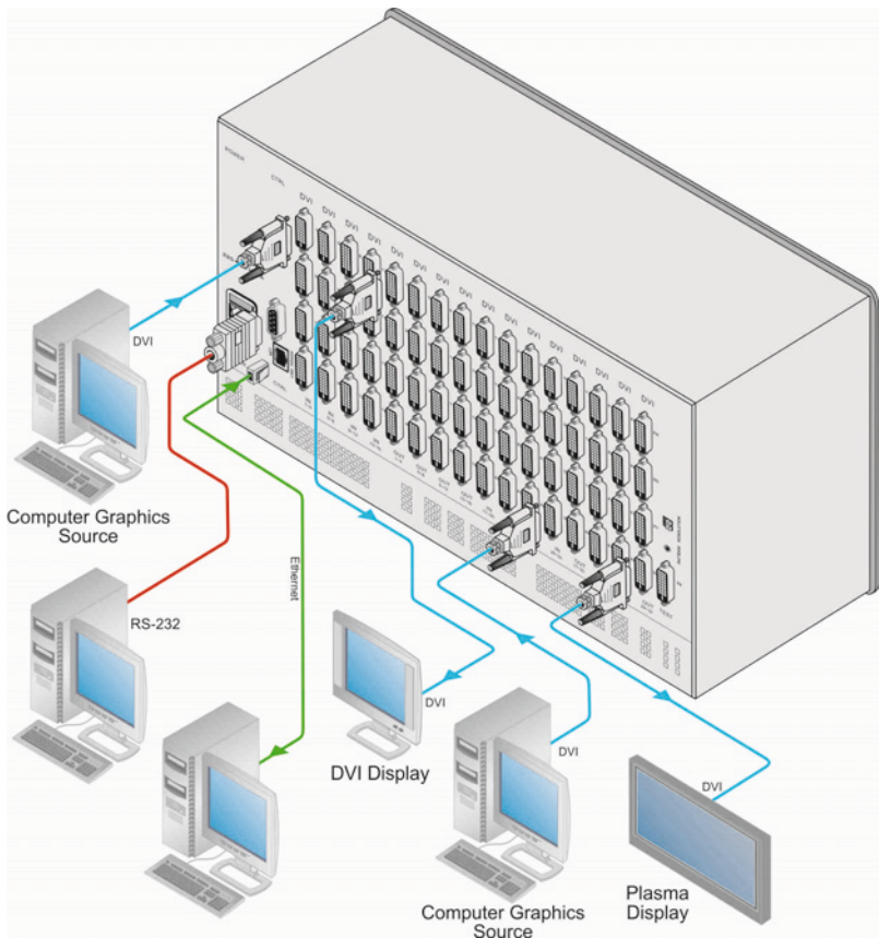
Figure 4: Connecting the VS-3232DN 32x32 Digital Matrix Switcher
