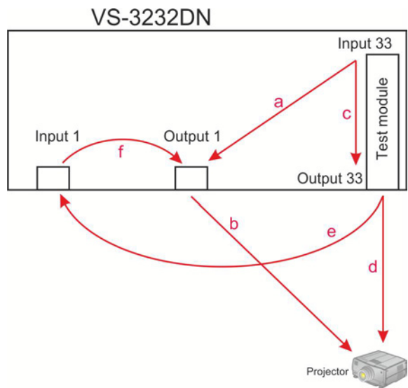
Figure 11: Signal Paths for Isolating Problems
