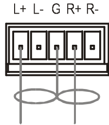
Figure 10: Connecting an Unbalanced Stereo Audio Output
