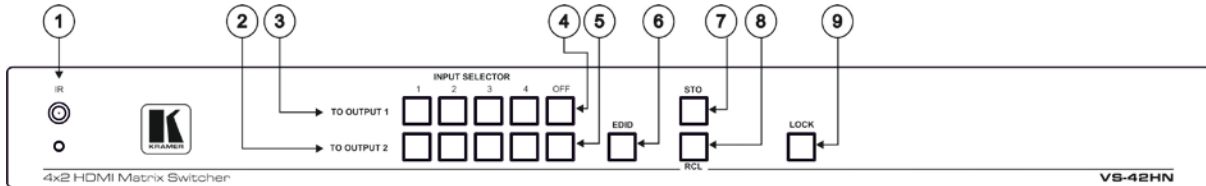
Figure 1: VS-42HN 4x2 HDMI Matrix Switcher Front Panel
