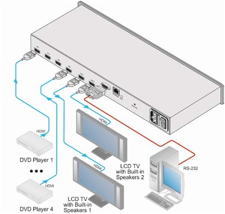
Figure 3: Connecting the VS-42HN 4x2 HDMI Matrix Switcher
