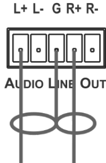
Figure 13: Connecting an Unbalanced Stereo Audio Acceptor to the Balanced Output
