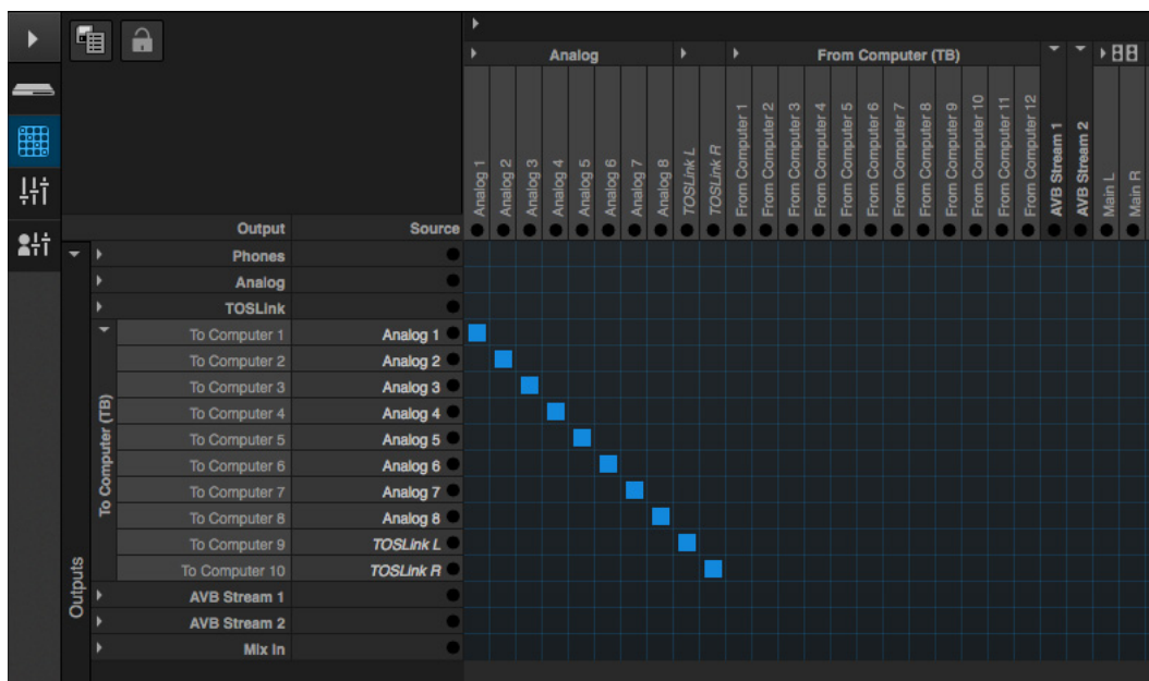
Figure 7-7: An example of routing physical inputs on the 8A to computer channels (for host audio software).
