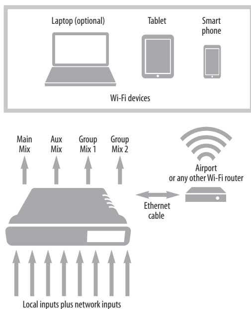
Figure 5-2: Using the 8A as a stand-alone mixer. This example demonstrates how you can control the mixer from several Wi-Fi devices.
