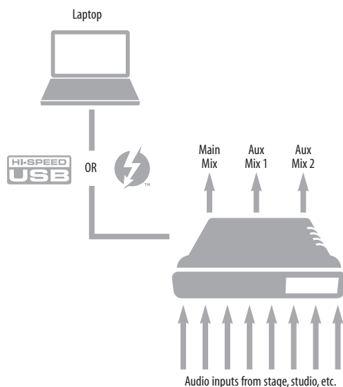
Figure 5-3: Using the 8A as an audio interface and mixer, simultaneously.
