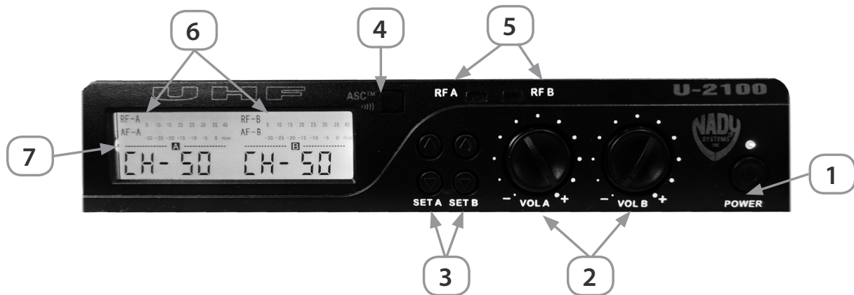
U-1100/U-2100 Receiver: Front View
