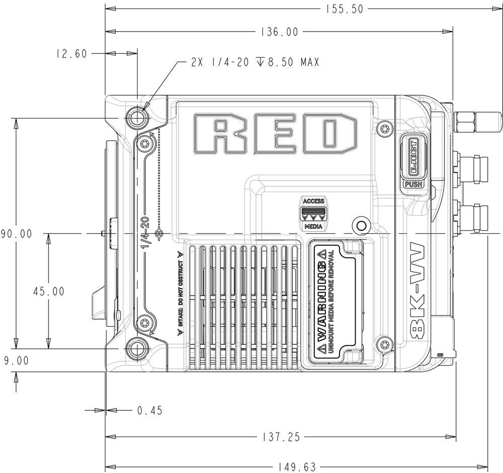
Figure: Camera Side View (Left)
