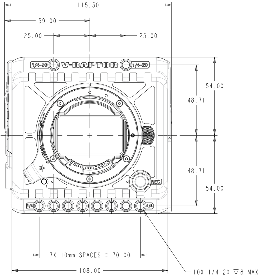
Figure: Camera Front View
