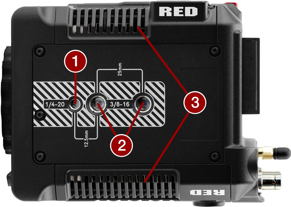
Figure: Camera Body Bottom Features
