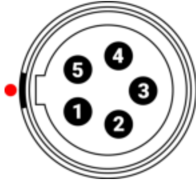
Figure: Front face of the female 5-Pin 00B audio connector (looking at the back of the camera).
