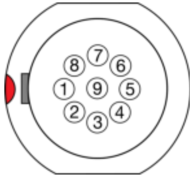
Figure: Front face of the female 9-contact Extension port (looking at the back of the camera).
