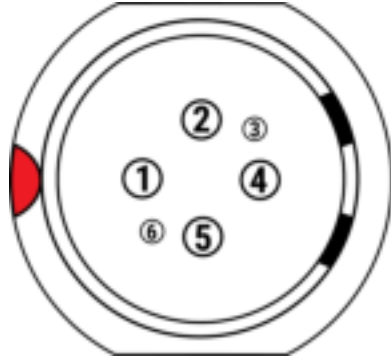
Figure: Front face of the male 6-Pin 1B DC power input connector (looking at the back of the camera).
