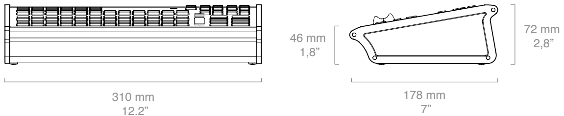
Figure 1: Technical drawing of Air Fly with key dimensions and layout details.
