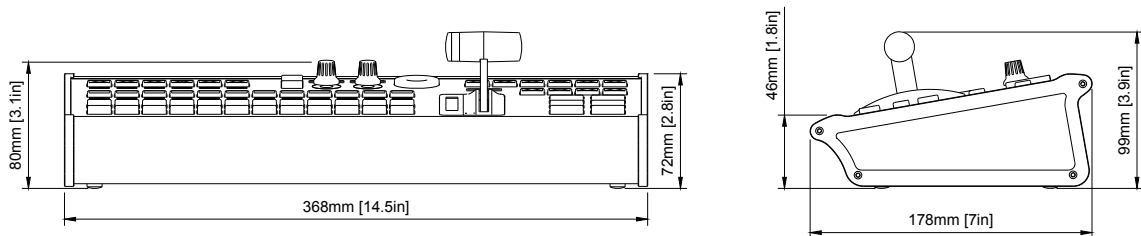
Figure 1: Technical drawing of Air Fly Pro with key dimensions and layout details.
