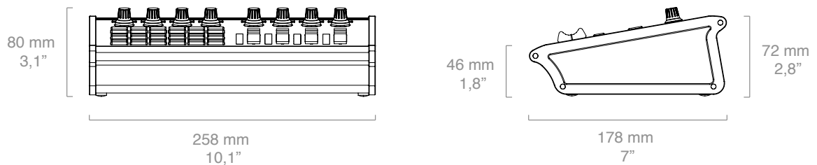
Figure 1: Technical drawing of Color Fly with key dimensions and layout details.
