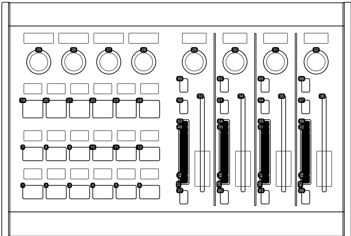
Figure 2: Diagram of hardware components for Color Fly with component IDs (HwC ID)
