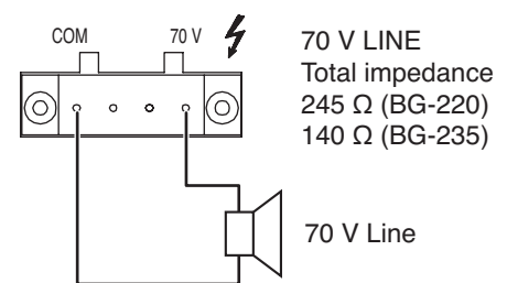
Speaker output terminal
