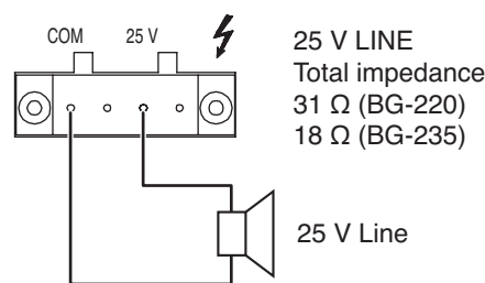
Speaker output terminal
