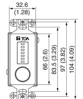
[Front View without panel]
