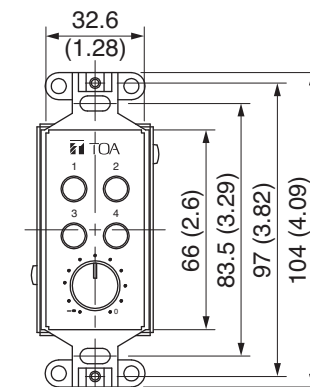
[Front View without panel]
